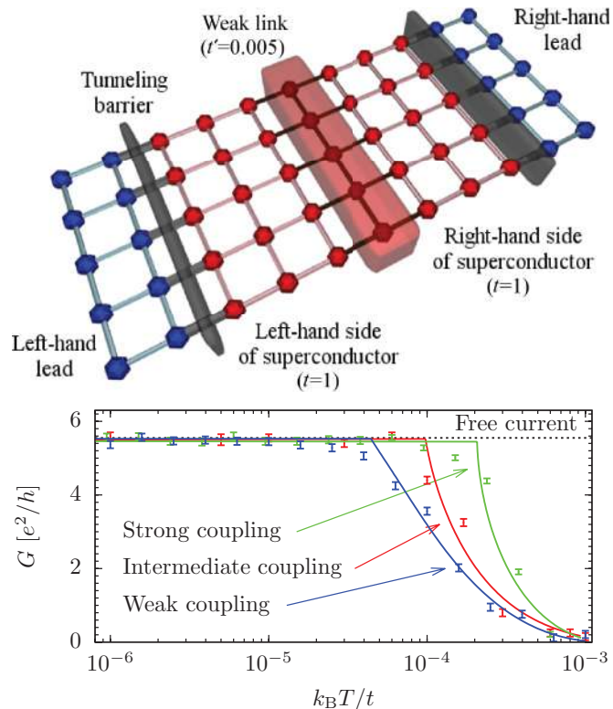
FIG. 3. (Color online) Upper: Setup to model the Josephson junction. Traversing the center of the SC region is a Josephson junction (opaque cuboid). The junction is modeled by the reduction of the matrix hopping elements to t' = 0.005 (brown interconnects) compared to t = 1 in the superconductor. The two metallic leads are shown on the far left and right (in blue), and the lead-superconductor tunneling barrier by the gray cuboids. Lower: The variation of conductance with temperature for the Josephson junction. Results of the numerical computation (points) and of the theoretical model (solid lines) are shown for a weak, intermediate, and strong coupling between the two superconductors.
