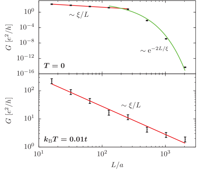
FIG. 5. (Color online) Fall in conductance with length in a noninteracting one-dimensional wire with disorder W = 0.2t at two different temperatures. The straight (red) trend lines show a linear drop off in conductance with length, and the curved (green) an exponential decay.
