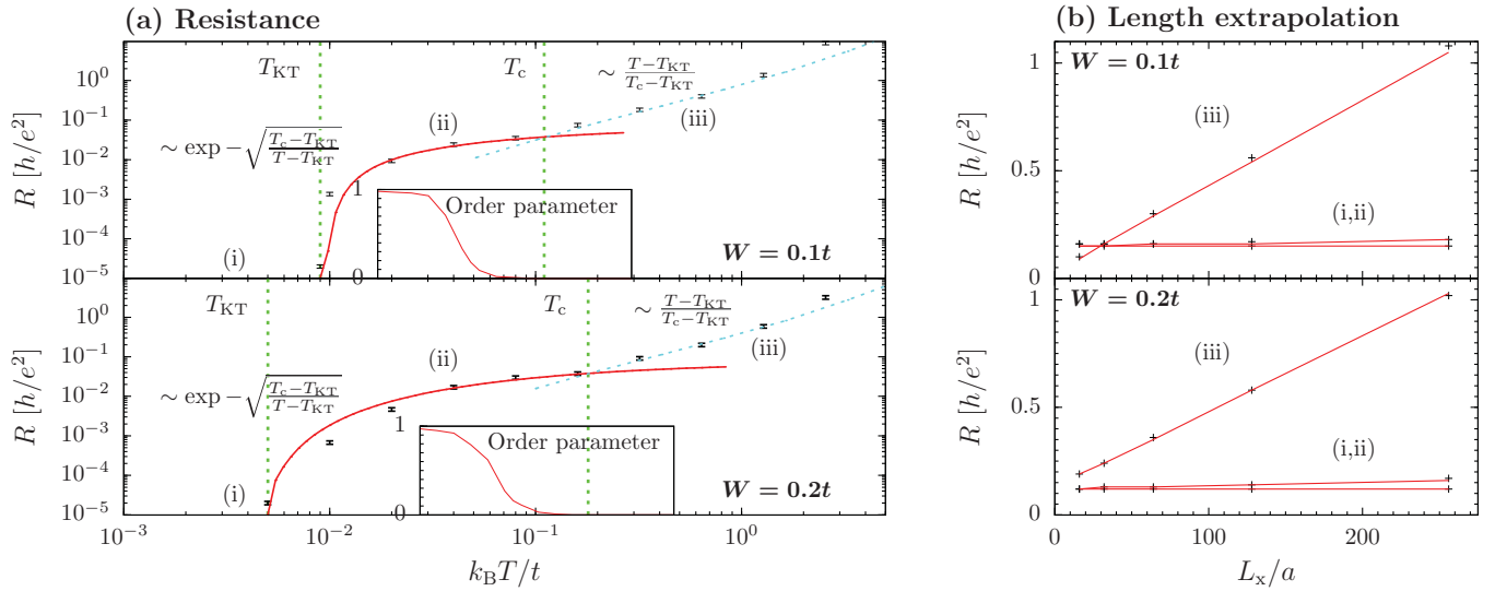
FIG. 6. (Color online) (a) Variation of resistance with temperature for two different values of disorder calculated numerically (points). The red solid line shows the theoretical low-temperature behavior, and the blue dotted line the theoretical high-temperature behavior. The dashed vertical green lines show the BKT T_{KT} and mean-field T_c temperatures. The insets show the variation of the superconducting order parameter U \langle c_\uparrow c_\downarrow \rangle renormalized by its T = 0 value. (b) Numerical results (black points) and the deduced linear length dependence (red solid line) of the resistance for three different temperatures (i) T < T_{KT} , (ii) T_{KT} < T < T_c , and (iii) T > T_c . The L \rightarrow 0 values correspond to the contact resistance, which is eliminated in the values plotted in (a).
