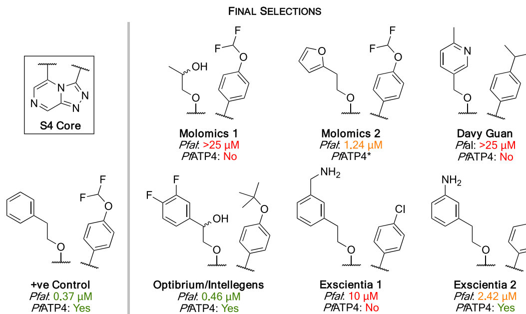
Figure 5. Six chosen suggested compounds for experimental validation. The predictions were synthesized (see the SI) and their potencies and MoAs (Figure S9) were experimentally validated. Three compounds were found to be active. *PfATP4 activity was not obtained for this compound.
